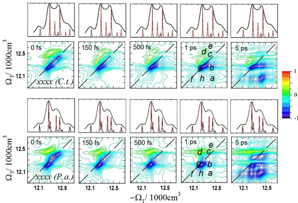
FIGURE 2 Simulated 2D ENC xxxx spectra of FMO from C.t. and P.a. for several time delays t_2 . The resolved diagonal and crosspeaks are illustrated ( a-h ). The linear absorption spectra ( top ) indicate the positions of single-exciton states.
